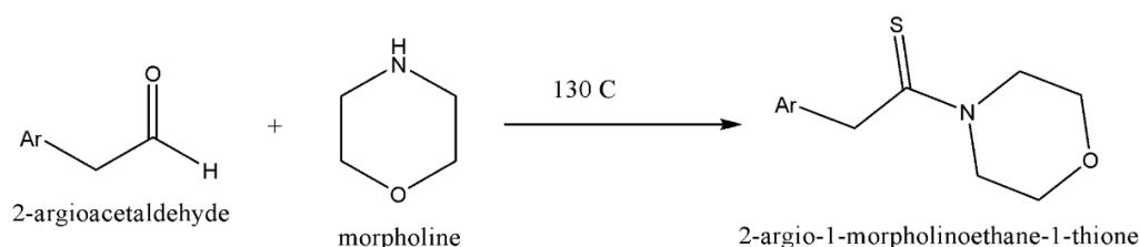
Figure 3. Synthesis of thioamides bearing an active methylene group via the Willgerdt-Kindler reaction ( Sarkis & Faisal, 1985 ).
