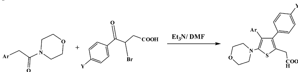
Figure 5. Synthesis of thiopheneacetic acids ( Jios et al., 2006 ).
