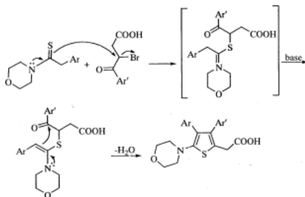
Figure 6. Scheme of Proposed mechanism for the synthesis of thiopheneacetic acids from aromatic thioamides.
