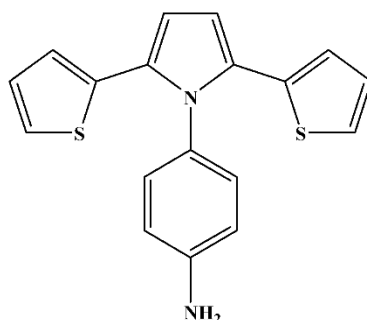
Figure 2. Chemical structure of di(thiophen-2-yl)-1H-pyrrol-1-yl phenylamine (Baudry et al., 1993).
