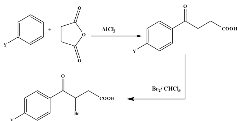
Figure 4. Synthesis of the acidic precursors (Martínez-Máñez & Sancenón, 2003).
