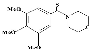
Figure 1. Chemical structure of Tritiozine, an analgesic and gastric acid antisecretory agent (Schroeder, 1955).
