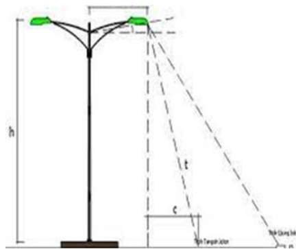
Figure 2. Distance From Lights to The Middle Of The Road (6)
